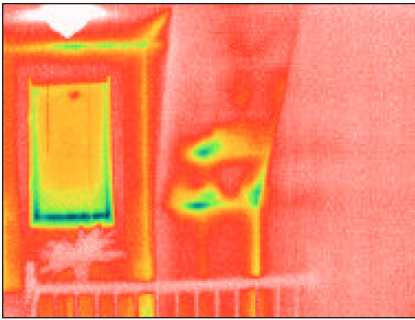
Image 3: The improperly installed fiberglass yields an irregular thermal pattern. The resulting cold spots commonly host wall stains or mold growth.
