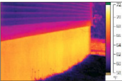
Image 6. In this example, the outside temperature was about equal to the inside temperature.
