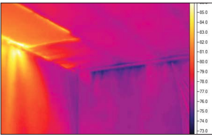
Image 10. Hot and cold thermal patterns appear next to each other in this photo.
